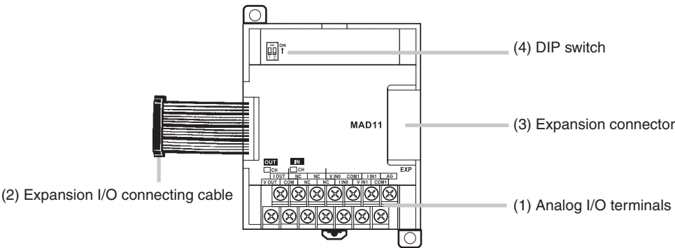
CP1W-MAD11/CPM1A-MAD11
