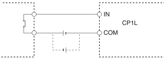
Contact output
