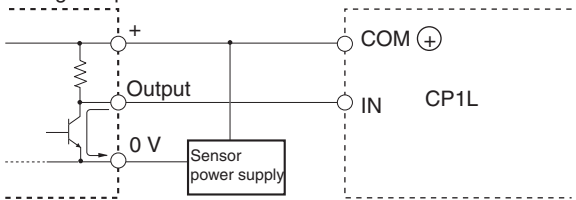
Voltage output
